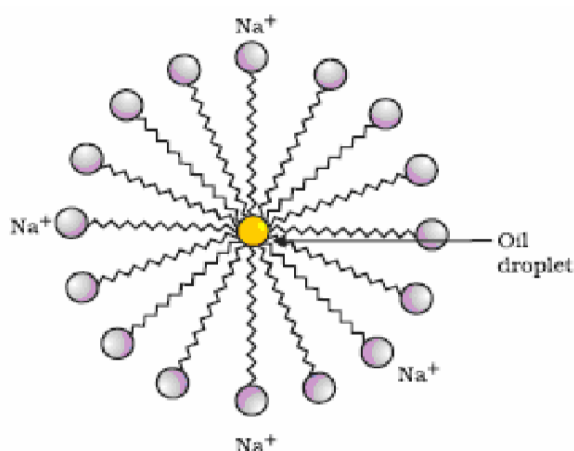
Formation of micelles
